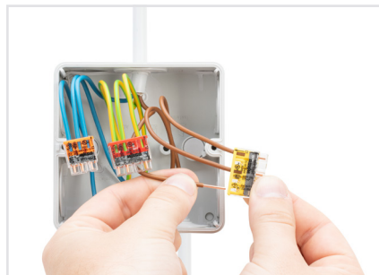
Termination: Insert the stripped conductor until it hits the backstop.
