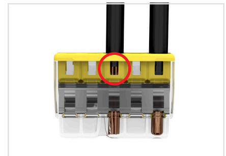
The transparent housing shows if conductors are fully inserted; within the coloured base, a clear port shows if the conductor's strip length is correct. Conductors are correctly stripped if the clear port shows no bare conductor on the unprinted connector side. Picture shows center conductor with exceeded strip length.
