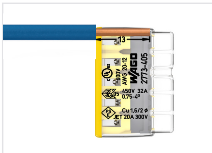
Strip solid or stranded conductor to 13 mm.
