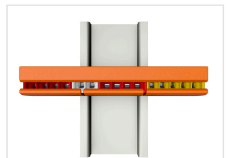
The mounting carrier also allows the connectors to be mounted on DIN-rails and used in control cabinets.
