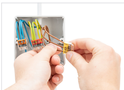
Removal: Hold solid conductor to be removed and twist alternately left and right while pulling the connector. Stranded wire: simply cut the wire close to the connector entry, strip it and insert into a new connector.
