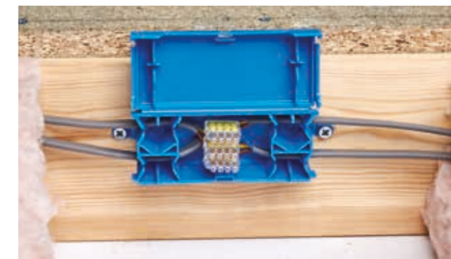
Lighting spur
