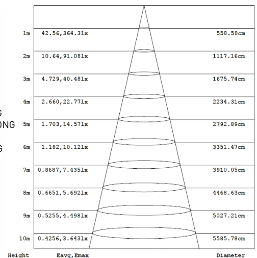
Diagram for RMU1420-40. Other diagrams available on request
