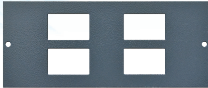
STO302 4 Way Data Plate 4 x 37x22mm LJ6C Module Cutouts
