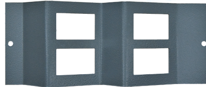
STO302/W 4 Way Data Wave Plate 4 x 37x22mm LJ6C Module Cutouts
