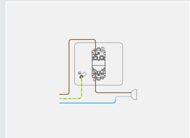
TYPICAL RETRACTIVE SWITCH CIRCUIT
