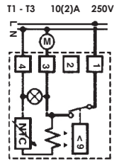
TH90 & TH90F - With normally closed contact (SPST)
