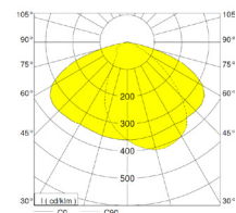
TYPICAL COUGAR LIGHT DISTRIBUTION DIAGRAM
