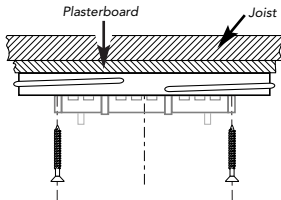
Figure 2 - Mounting Ceiling Rose base
