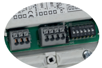
Terminals and dip-switch selection
