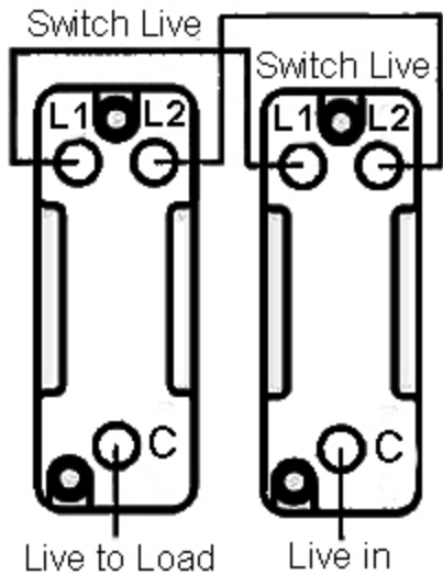
Alternative 2 Way Switching
