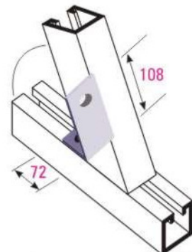
Acute Angle Bracket WEIGHT 0.33 KG.
