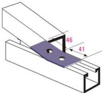
Obtuse Angle Bracket WEIGHT 0.13 KG.
