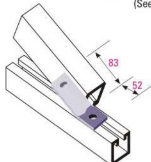
Obtuse Angle Bracket WEIGHT 0.25 KG.
